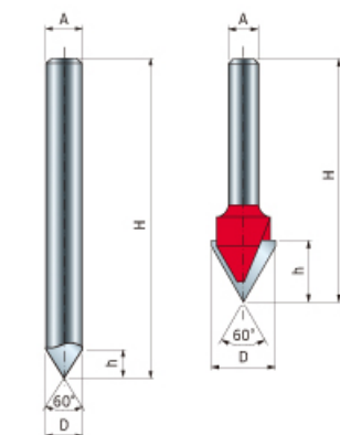
● 솔초경비트 Solid Carbide Bit
